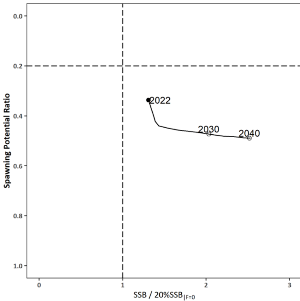
Figure 6-1. “Future Kobe Plot” of projection results for Pacific bluefin tuna Thunnus orientalis from Scenario 1 in Table 4-2. Vertical and horizontal dashed lines show 20\%SSB_{F=0} (which corresponds to the second biomass rebuilding target) and the corresponding fishing mortality that produces SPR, respectively.
