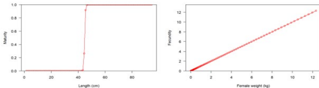
Figure 9-22. Maturity-at-length (FL; left) and fecundity-at-weight (right) used in the stock assessment model.
