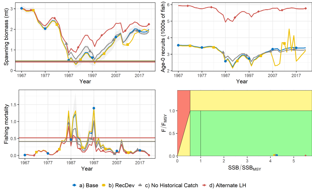
Figure 9-55. Alternative model runs showing differences in spawning biomass, recruitment, fishing mortality, and a Kobe plot of the final year stock status (in order from left to right) b) with recruitment deviations, c) without historical catch data (model starts in 1986), and d) with an alternate life history parameter source (longevity from StepwiseLH).
