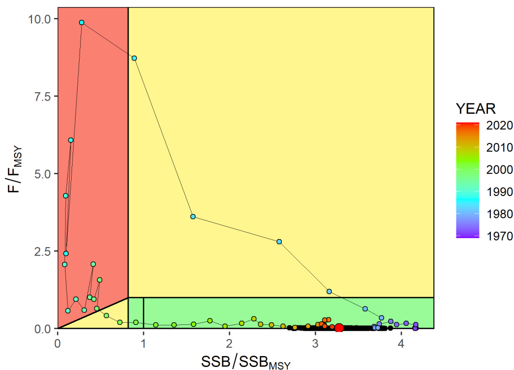
Figure 9-149. Kobe plot representing the trend in relative fishing mortality and spawning stock biomass between 1969 and 2021 with their associated biological reference areas (red: overfished and overfishing, yellow: overfishing or overfished, green: no overfishing and not overfished). The large red dot indicates median stock status in 2021 and the black dots are one thousand Monte Carlo draws from the stock status distribution to represent the uncertainty around the final year status.
