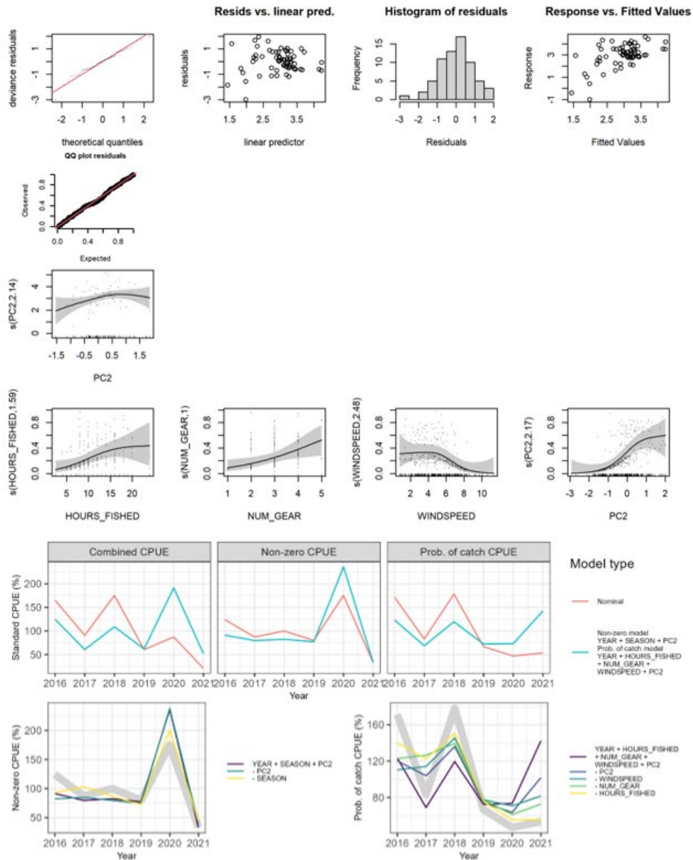
Figure 8-10. CPUE model diagnostics for Etelis coruscans . The first two rows contain residual plots followed by partial effect plots of smooth terms for the non-zero catch and probability of catch models. Row 5 shows plots comparing nominal CPUE vs. the best CPUE model, while the last row shows plots comparing progressively simpler version of the best model.
