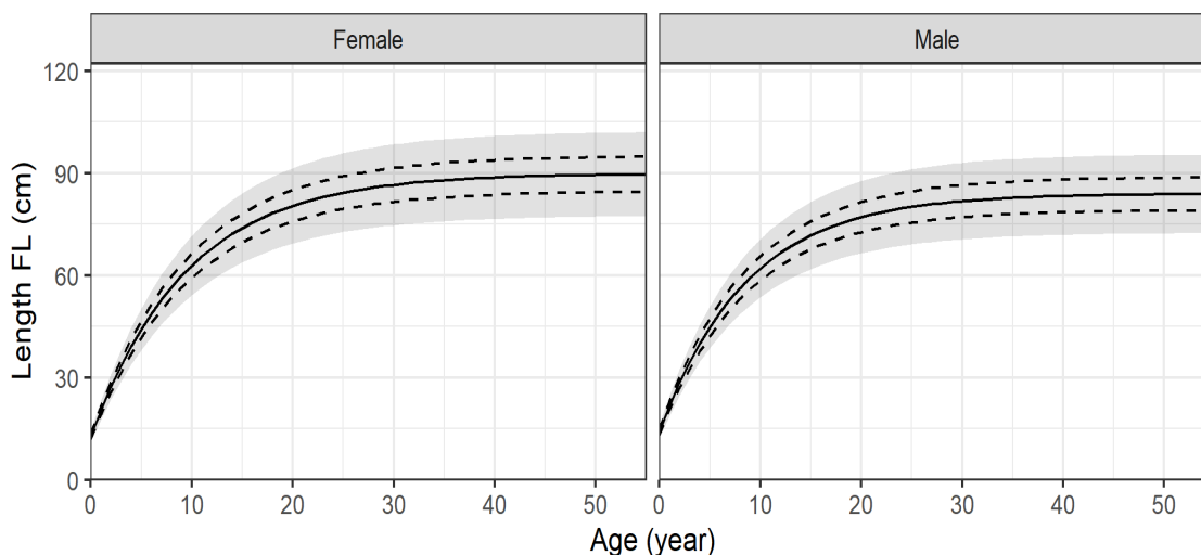
Figure 9-59. Growth curve following a Von Bertalanffy model with 95% confidence intervals associated with the CV Linf parameter. The central growth plateau (solid line) and the two secondary ones (dashed lines) used in the model are also displayed.
