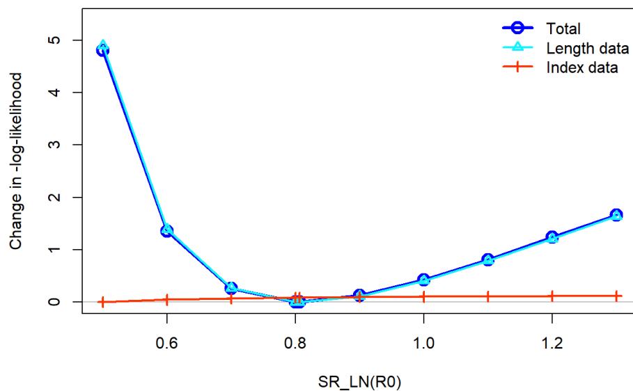
Figure 9-68. Profiles of the change in negative log-likelihoods relative to the minimum value of each component for the different likelihood components affecting the unfished recruitment parameter ( R_0 ) in log-scale.
