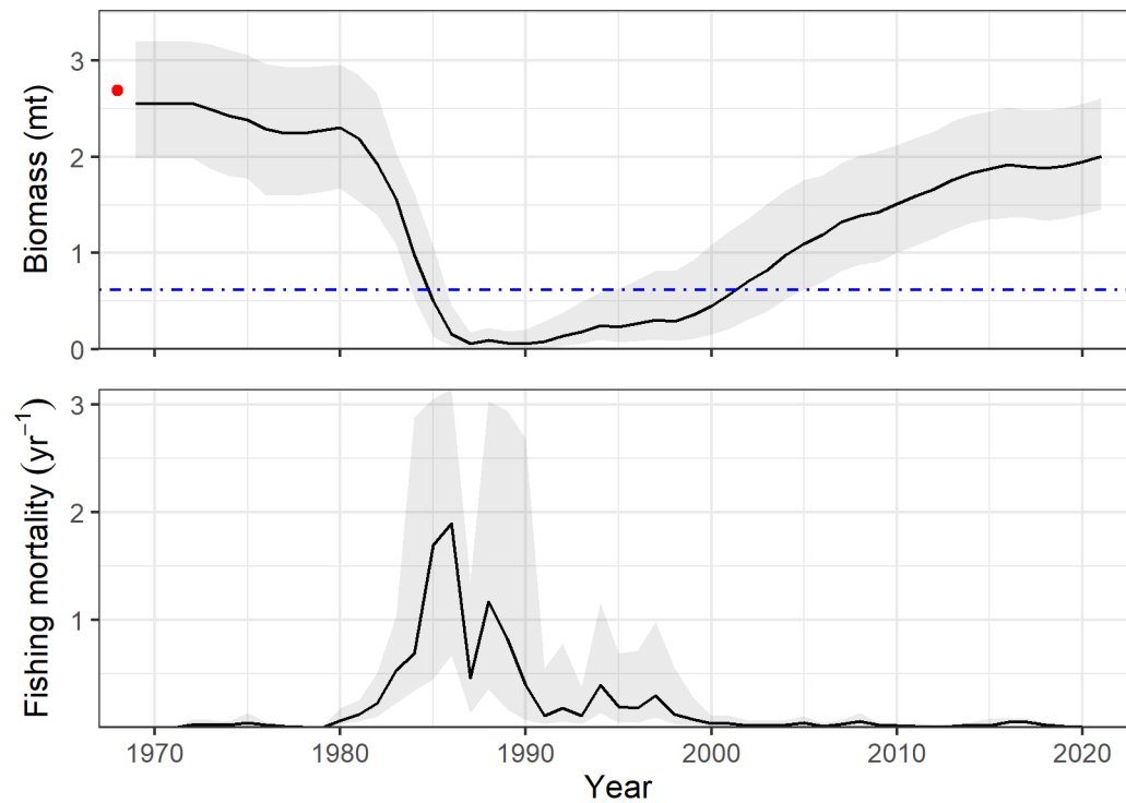
Figure 9-147. Time series of spawning biomass (solid line) with its 95% confidence interval and SSB_0 estimate (red dot; top panel). The dot-and-dash blue line shows the spawning biomass at the MSST reference point ( SSB_{MSST} ). Time series of fishing mortality rate with its 95% confidence intervals (bottom panel).
