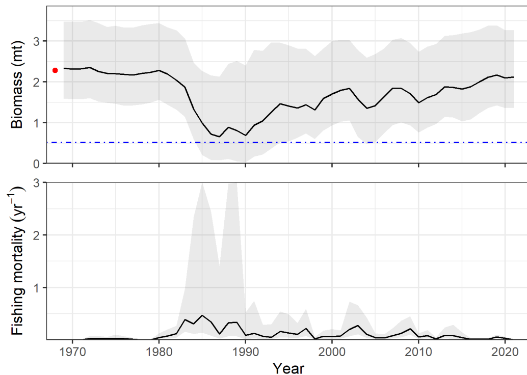
Figure 9-167. Time series of spawning biomass (solid line) with its 95% confidence interval and SSB_0 estimate (red dot; top panel). The dot-and-dash blue line shows the spawning biomass at the MSST reference point ( SSB_{MSST} ). Time series of fishing mortality rate with its 95% confidence intervals (bottom panel).
