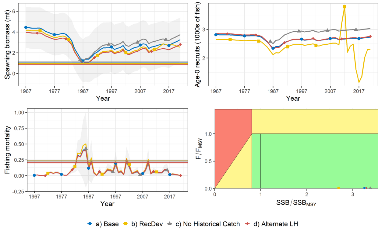
Figure 9-132. Alternative model runs showing differences in spawning biomass, recruitment, fishing mortality, and a Kobe plot of the final year stock status (in order from left to right) b) with recruitment deviations, c) without historical catch data (model starts in 1986), and d) with an alternate life history parameter source ( L_{mat} from Brouard 1985).
