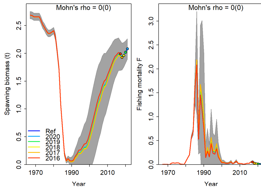
Figure 9-146. Retrospective analysis of spawning biomass (left) and fishing mortality (right) consisting of 5 reruns of the base case model each fitted with one less year of data from the base case model (blue line).
