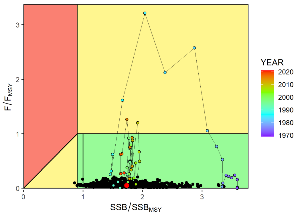
Figure 9-72. Kobe plot representing the trend in relative fishing mortality and spawning stock biomass between 1969 and 2021 with their associated biological reference areas (red: overfished and overfishing, yellow: overfishing or overfished, green: no overfishing and not overfished). The large red dot indicates median stock status in 2021 and the black dots are one thousand Monte Carlo draws from the stock status distribution to represent the uncertainty around the final year status.
