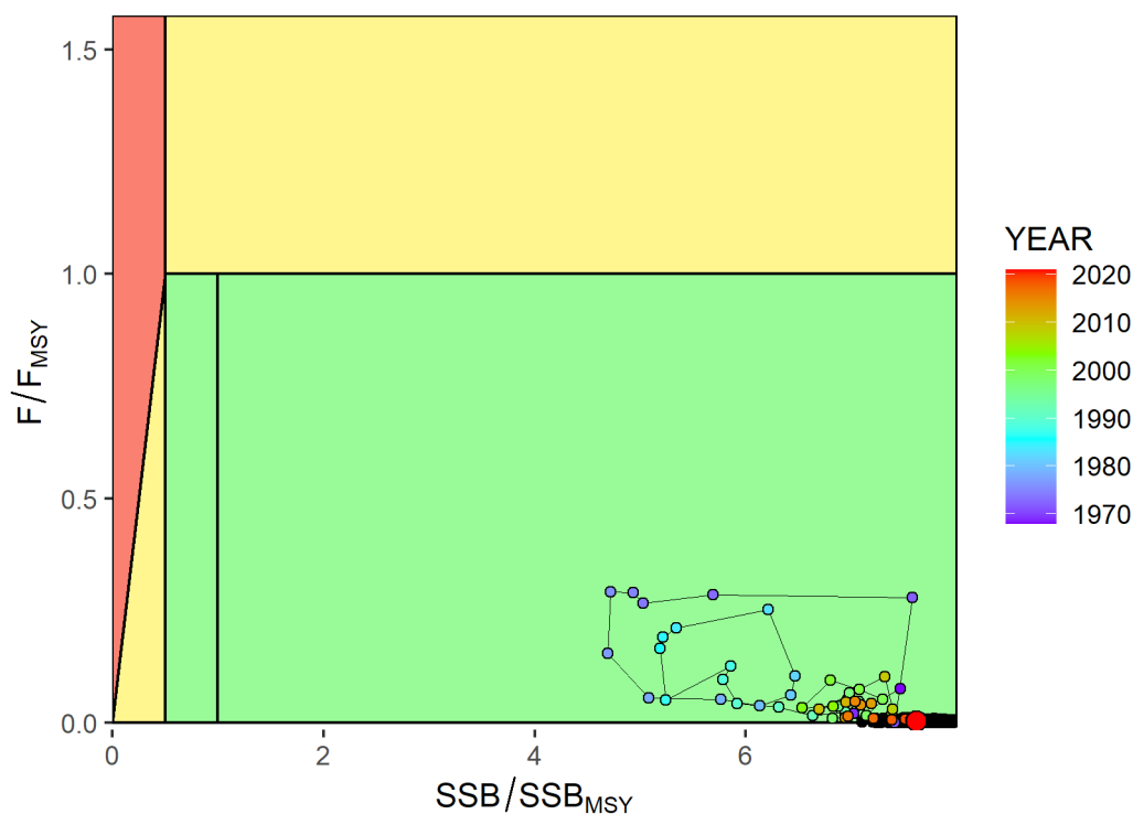
Figure 9-111. Kobe plot representing the trend in relative fishing mortality and spawning stock biomass between 1969 and 2021 with their associated biological reference areas (red: overfished and overfishing, yellow: overfishing or overfished, green: no overfishing and not overfished). The large red dot indicates median stock status in 2021 and the black dots are one thousand Monte Carlo draws from the stock status distribution to represent the uncertainty around the final year status.
