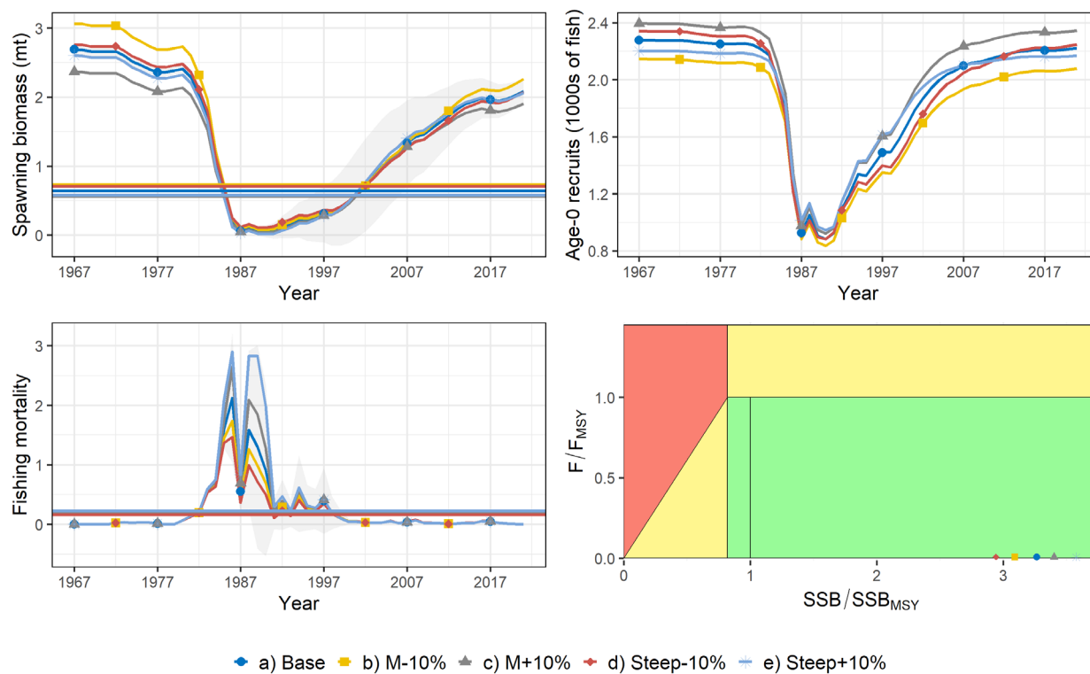
Figure 9-150. Alternative model runs showing differences in spawning biomass, recruitment, fishing mortality, and a Kobe plot of the final year stock status (in order from left to right) under moderate life-history parameter variation (plus and minus 10% of base parameter values).
