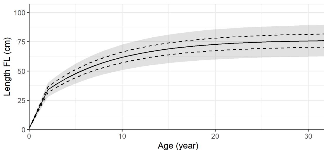
Figure 9-21. Growth curve following a Von Bertalanffy model with 95% confidence intervals associated with the CV Linf parameter. The central growth plateau (solid line) and the two secondary ones (dashed lines) used in the model are also displayed.
