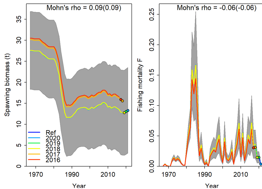
Figure 9-69. Retrospective analysis of spawning biomass (left) and fishing mortality (right) consisting of 5 reruns of the base case model each fitted with one less year of data from the base case model (blue line).
