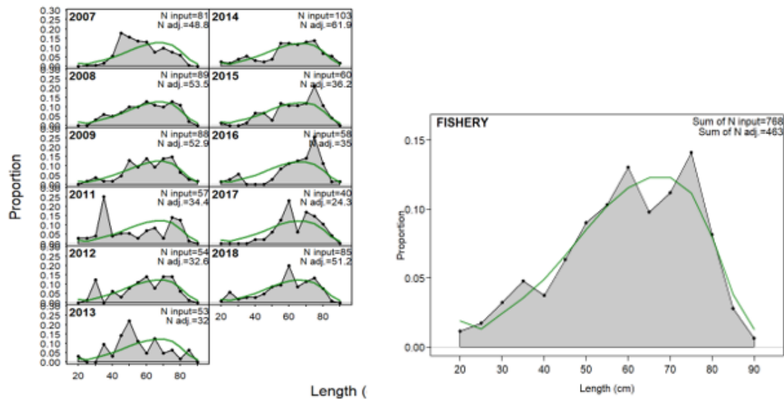
Figure 9-67. Observed (gray area) vs. expected (green line) abundance-at-length from bottomfishing catch by year (left) and overall (right).
