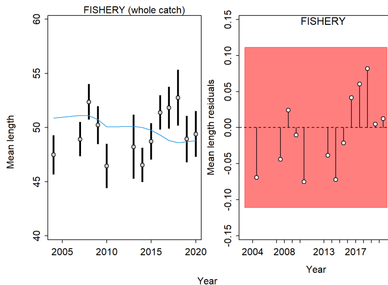
Figure 9-27. Observed (open dots) vs expected (blue line) mean length by year with standard deviations intervals (left). Mean length residuals by year with the background color indicating the result of the Runs test (right panel; green=pass, red=fail). The width of this colored area represents three residual standard deviations (points falling outside this area are colored in red). The root mean square error (RMSE) is 0.05.
