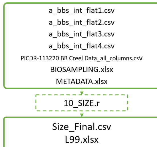
Figure 8-3. Data (solid boxes) and scripts (dashed boxes) used to generate the final size data used in our SS models.
